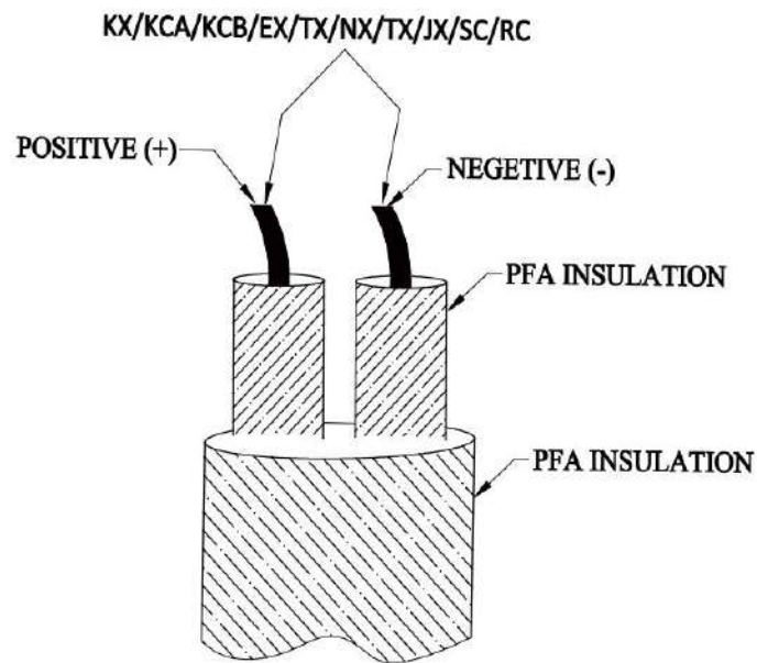
THERMOCOUPLE HIGH TEMPERATURE CABLE
