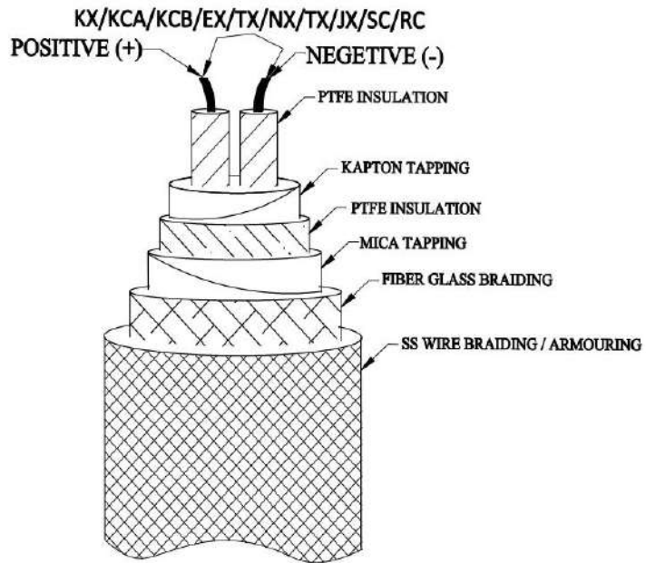
THERMOCOUPLE HEAT RESISTANCE CABLE
