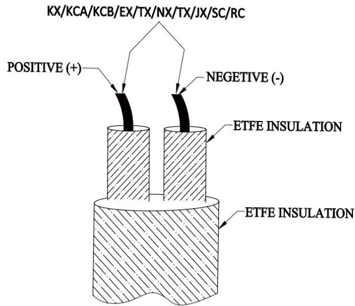
THERMOCOUPLE HIGH TEMPERATURE CABLE
