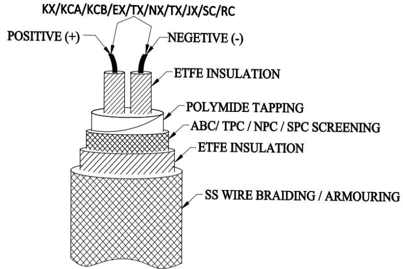
THERMOCOUPLE HIGH TEMPERATURE CABLE
